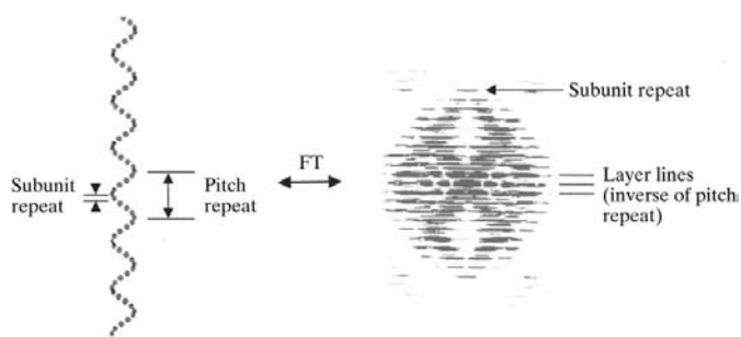
Figure 9 Helical diffraction. A helix can be considered as a 1D crystal, since it has a repeating structure along the axis giving rise to a set of layer lines in the diffraction pattern. If the symmetry of the helix is known, a full 3D reconstruction can be calculated from the untilted filament transform, since the subunit is imaged at different angles about the filament axis. The example shown is for the case of a helix with an integral number of subunits per helical pitch repeat.
