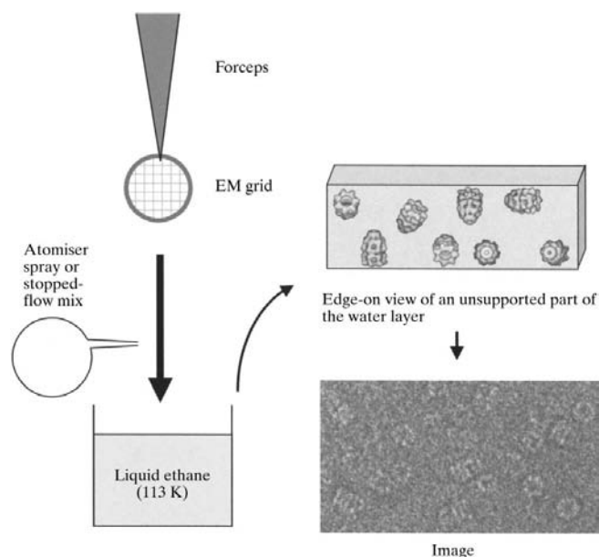
Figure 5 Vitrification of cryo-EM specimens and time-resolved cryo-EM. A cryo-EM grid with a thin film of solution is plunged into liquid ethane for vitrification. Time-resolved experiments are possible by spraying a reagent onto the grid just before it enters the ethane, using an atomiser. A time resolution of several milliseconds can be achieved. To the right is a schematic view of a part of the frozen water layer, with macromolecules trapped in different orientations. Bottom right, part of a cryo-EM image showing weak and noisy views of the complexes.
