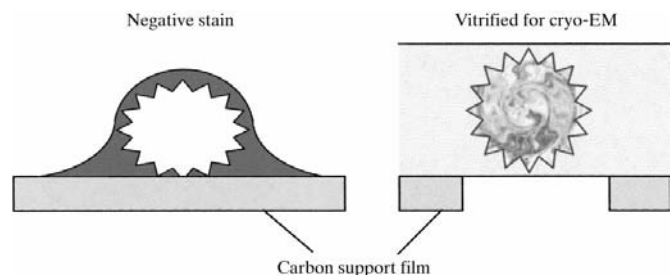
Figure 4 Negative-stain and cryo-EM. A virus particle on a carbon support film is shown in schematic side view. The particle is outlined with good contrast by heavy-metal stain, but is somewhat flattened by the accompanying dehydration. It is preserved in the native hydrated state in the cryo-sample but the protein–ice contrast is very low. In order to maximize the contrast, the cryo-specimen is imaged over holes in the carbon support film.
