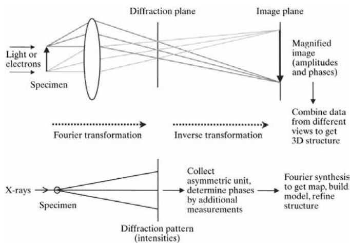
Figure 3 The relationship between imaging and diffraction. A simplified schematic view of imaging and diffraction shows that the waves scattered by the specimen form a Fourier transform, observed as a diffraction pattern. The objective lens in a microscope recombines the scattered waves in an inverse transformation, forming the magnified image. In the diffraction experiment, only the diffracted intensities are recorded and the lost phase information must be retrieved by other methods.
