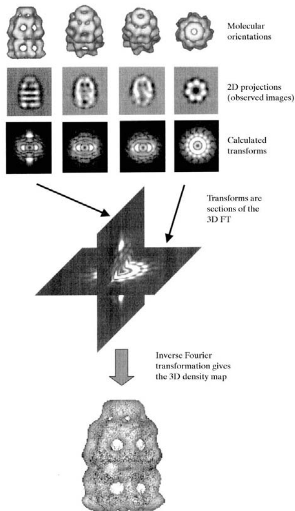
Figure 2 The principle of 3D reconstruction from 2D projections. A set of four different molecular orientations, displayed as rendered iso-surfaces, are shown above their corresponding 2D projections. Real cryo-EM images are very noisy versions of these projections. The Fourier transform of each projection, shown below the projections, is a section through the 3D Fourier transform of the structure (DeRosier & Klug, 1968). The 3D transform is represented by two intersecting transform sections, derived from the side and end views of the structure. Once enough sections are available, the full 3D transform can be interpolated and inverse transformed into a 3D density map. The map is shown with the backbone of the structure to emphasize the fact that the full 3D density is obtained, including internal features. Surface rendering is generally used to represent such maps when the resolution is insufficient to provide an atomic model of the structure.
