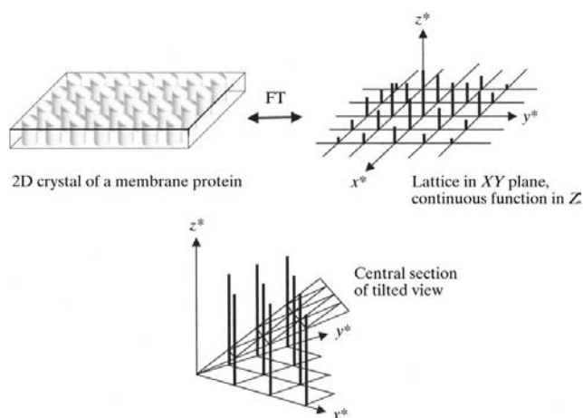
Figure 6 Data-collection geometry for 2D crystals. Each lattice line will have a continuously varying amplitude and phase along its Z coordinate. The tilted views sample the lattice lines at different heights in Fourier space. Most of the 3D FT can be determined by combining these sections derived from different tilt views in projection. However, in EM of 2D crystals there is a missing cone of information because the maximum tilt angle of the crystal is limited to about 60^\circ . Figure adapted from Amos et al. (1982).
