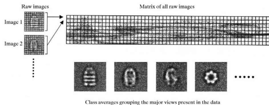
Figure 10 Image classification by multivariate statistical analysis. A large set of images is aligned to a common centre and then assembled into a matrix in which each row contains all the pixel values of a single image. Each raw image forms a row of the matrix. The first two images of a series and a small part of the matrix are shown. The eigenvectors of this matrix are difference images that represent the principal components of variation in the data set. Each image can then be represented by the average image \pm a series of difference components. Similar images are classified into subgroups on the basis of the coefficients of these components. Similar average of each subgroup gives an image with a greatly improved signal-to-noise ratio.
